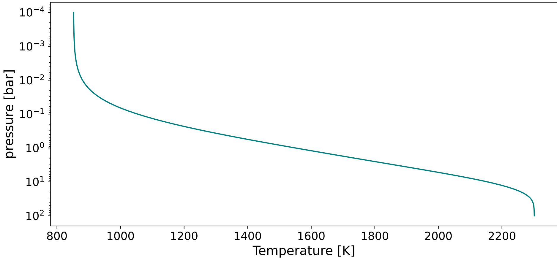
Line et al. (2013) T-p Profile
