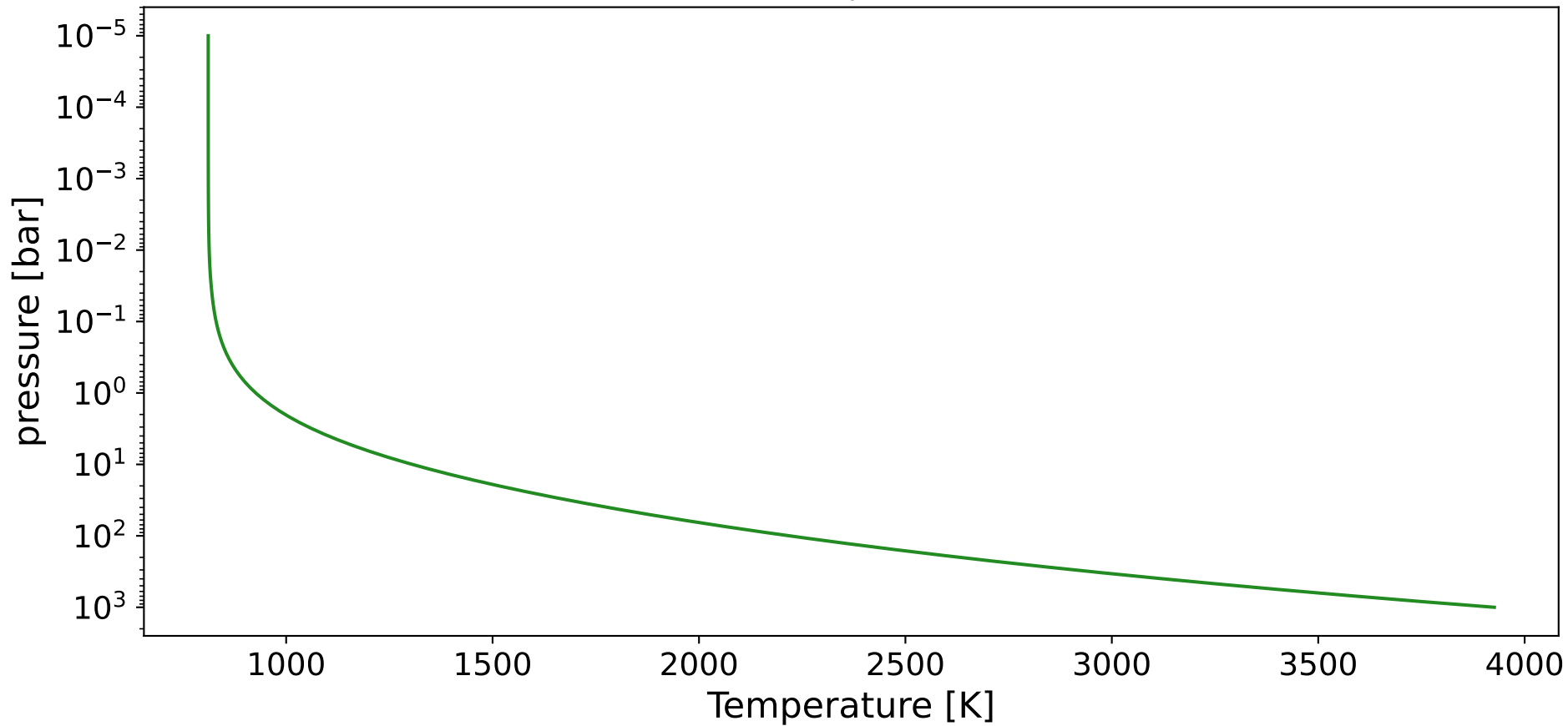
Milne T-p Profile
