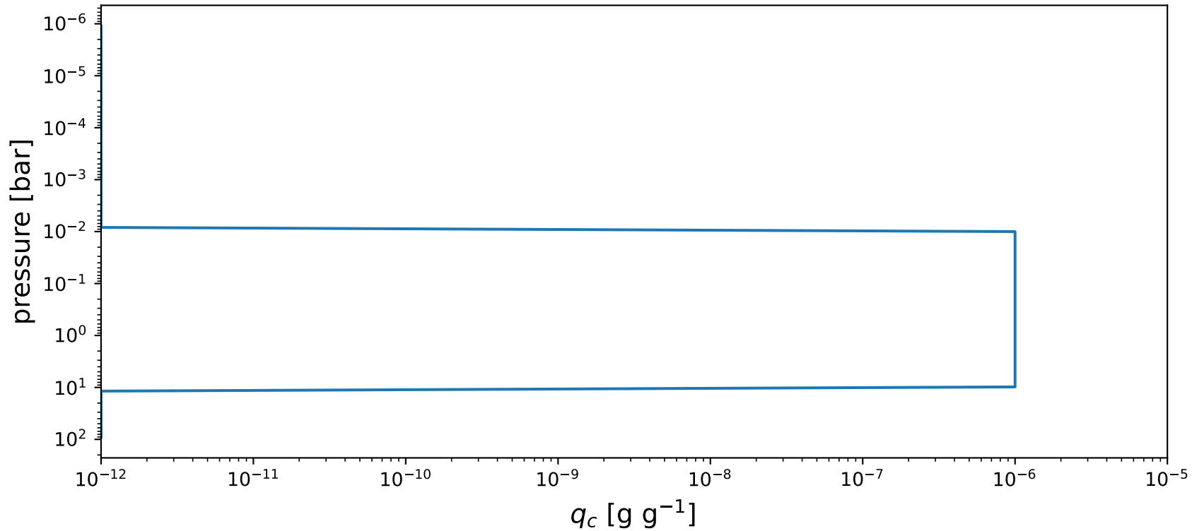
Slab Cloud Profile (floored at 10^{-12} for log-x)
