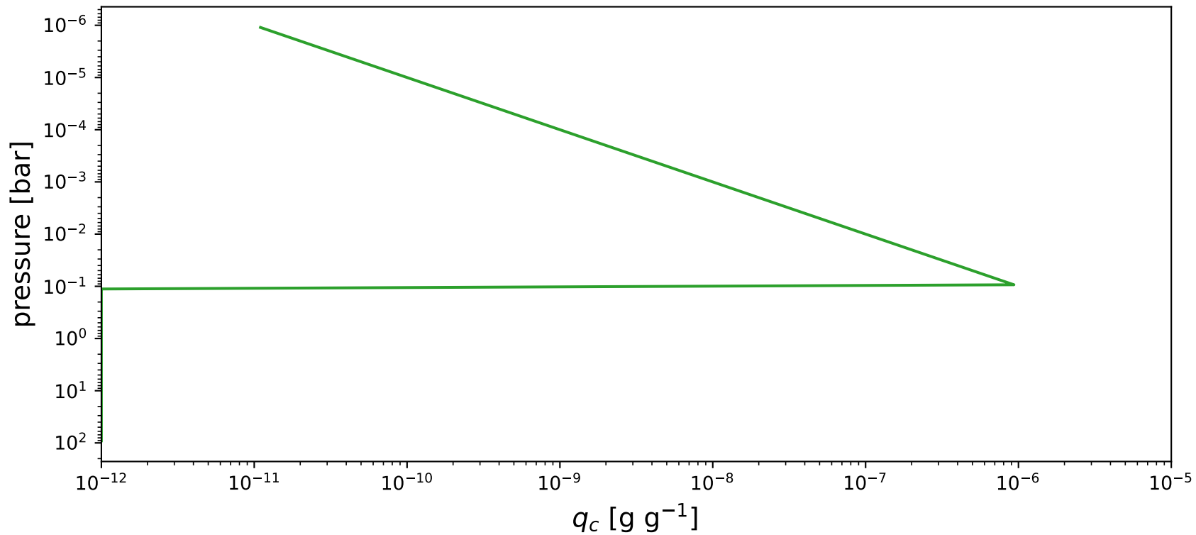
Exponential Decay Cloud Profile (floored at 10^{-12} for log-x)
