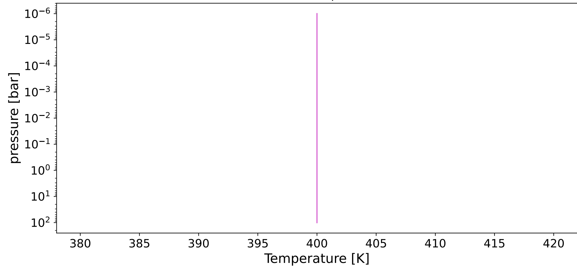
Isothermal T-p Profile
