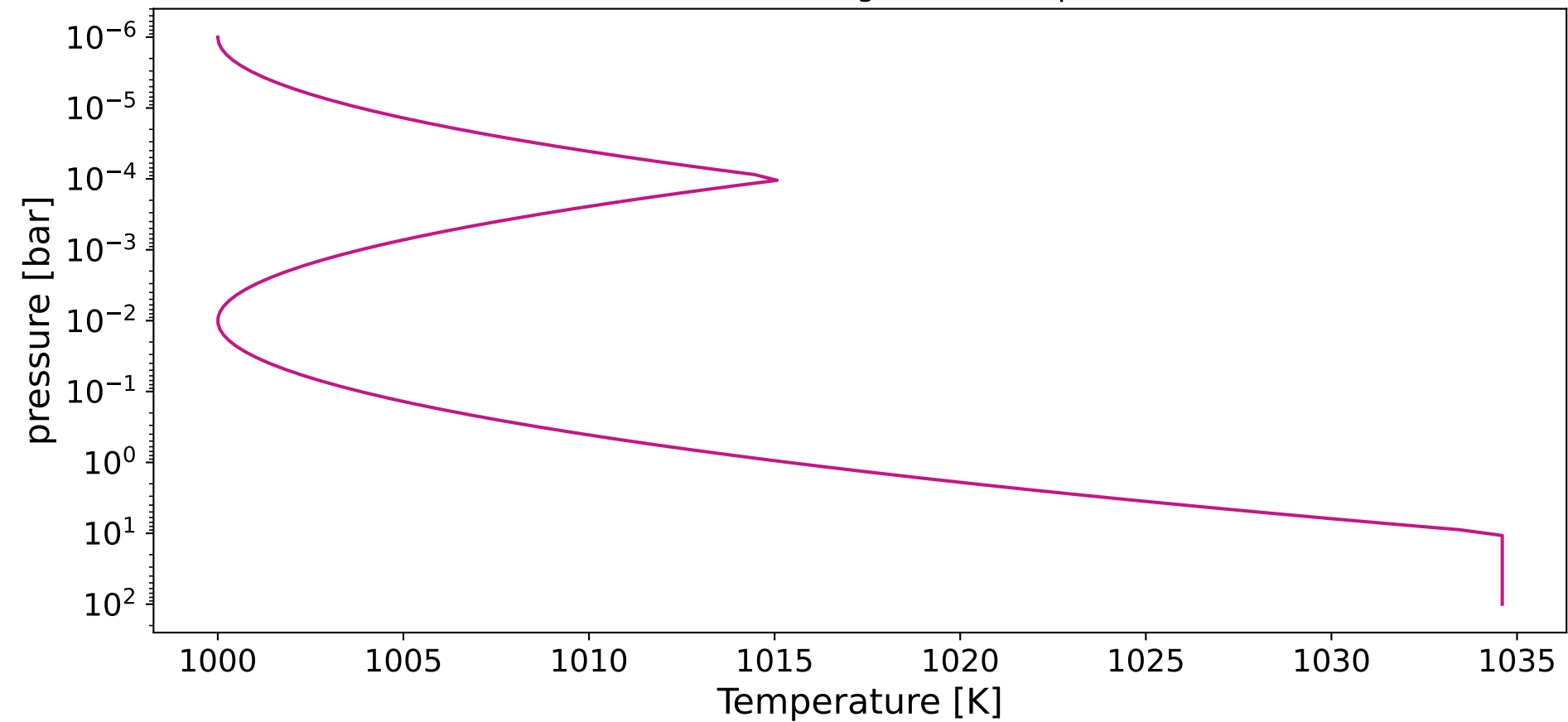
Madhusudhan & Seager (2009) T-p Profile
