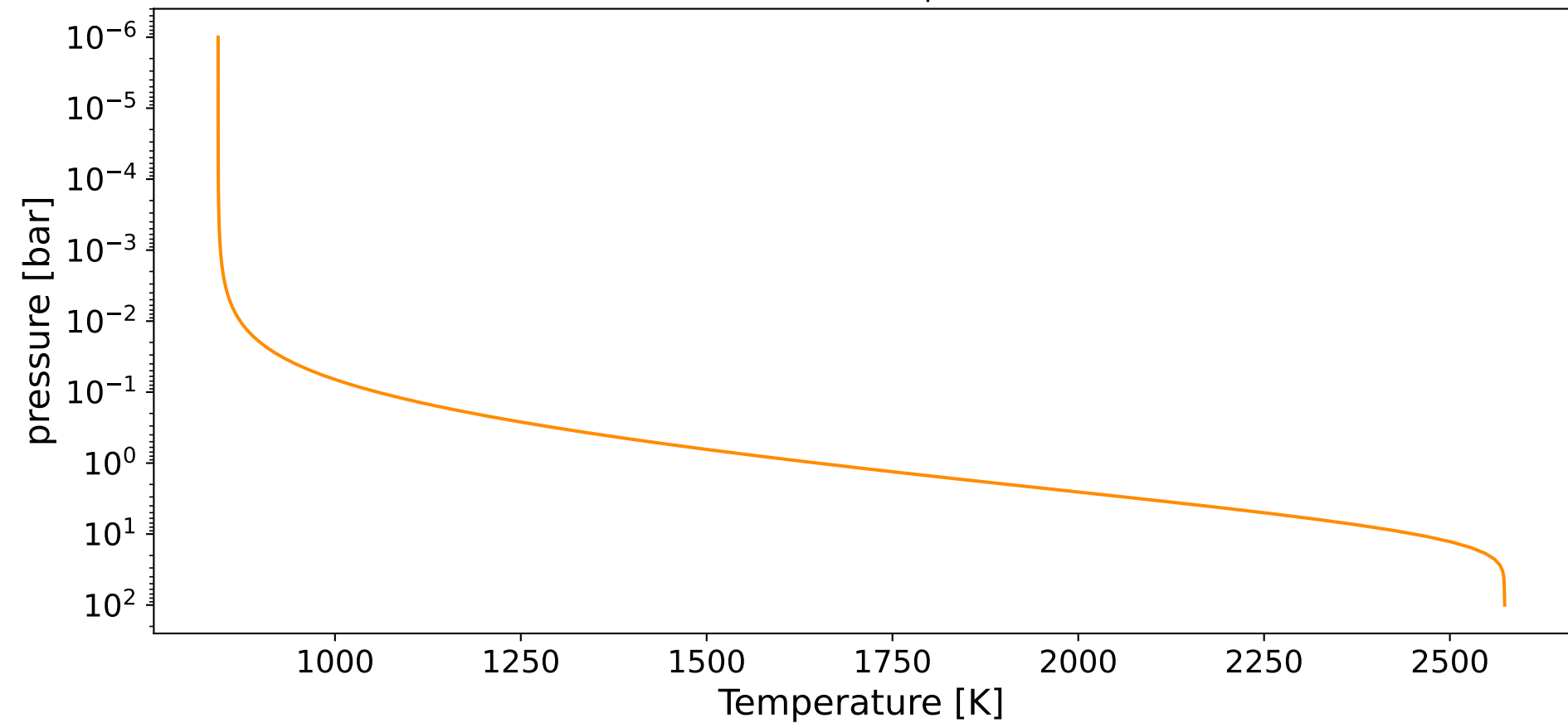
Guillot (2010) T-p Profile
