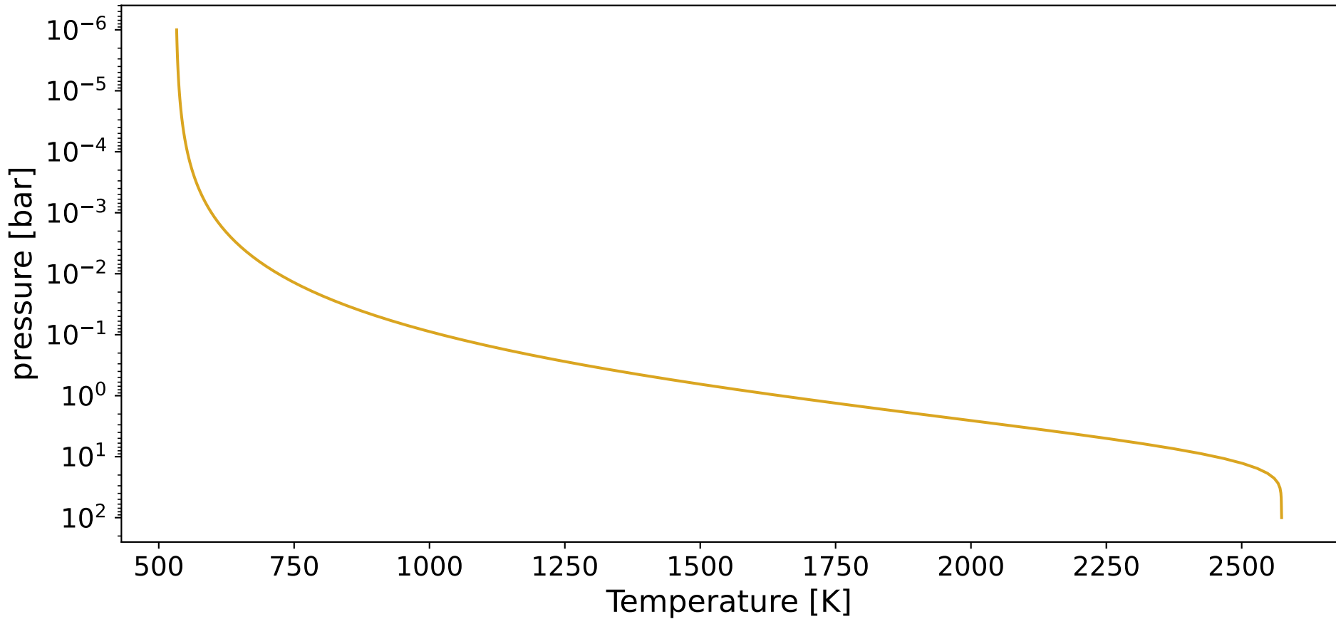
Modified Guillot T-p Profile
