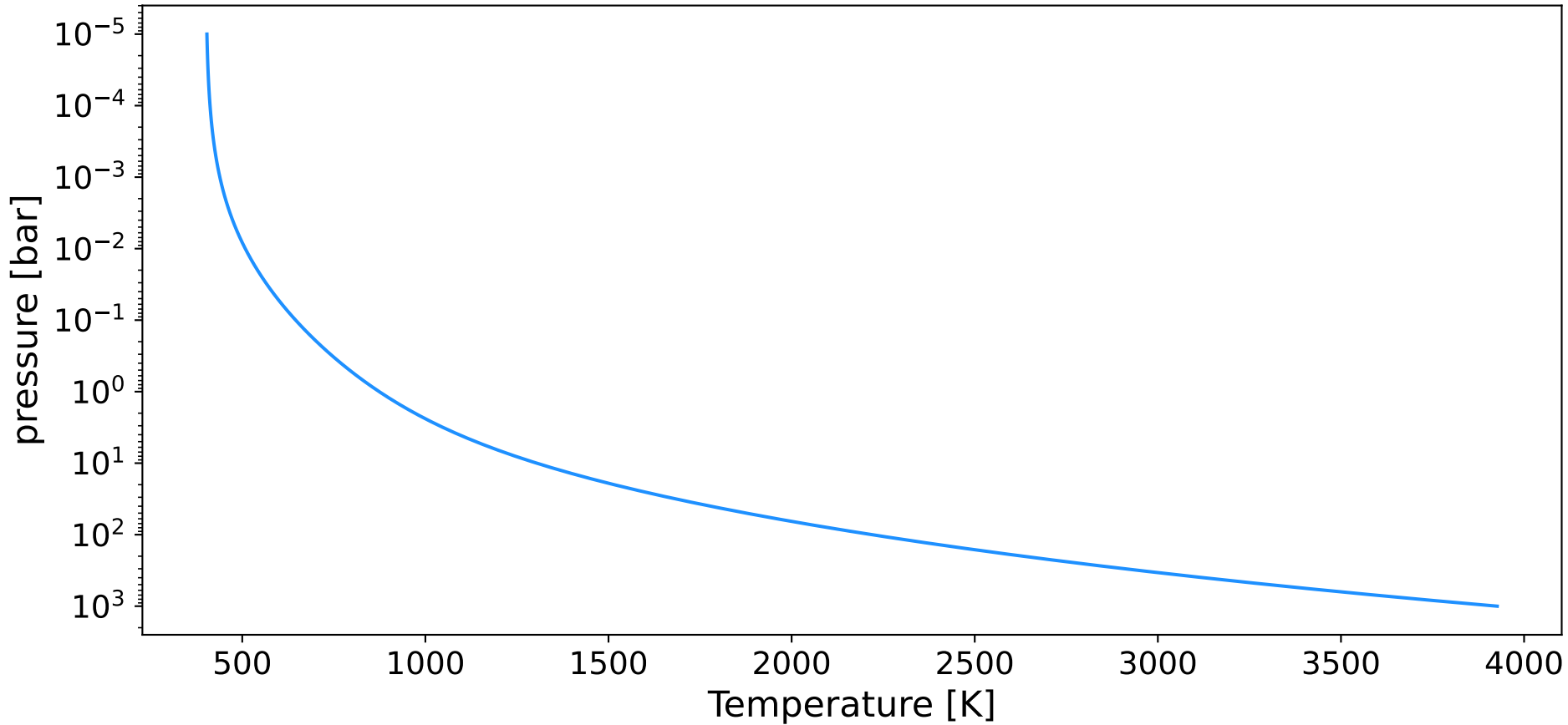
Modified Milne T-p Profile
